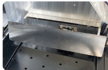
The print head anti-collision system can effectively prevent the printhead from being damaged during printing and ensure safety
